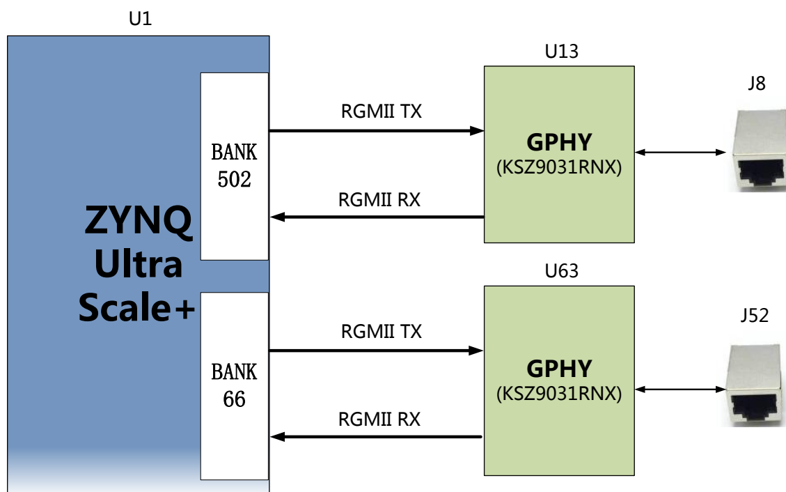
Figure 3-5-1: ZYNQ PS system and GPHY connection diagram
