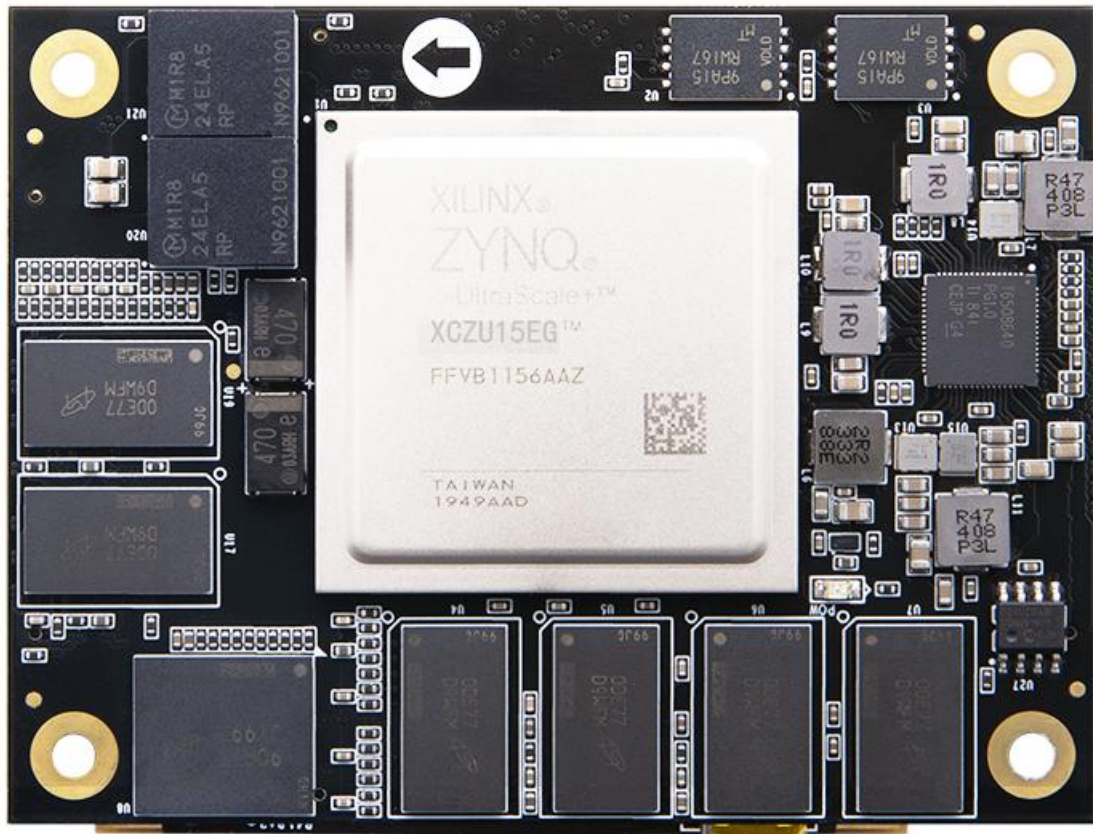
Figure 2-1-1: ACU15EG Core Board (Front View)
