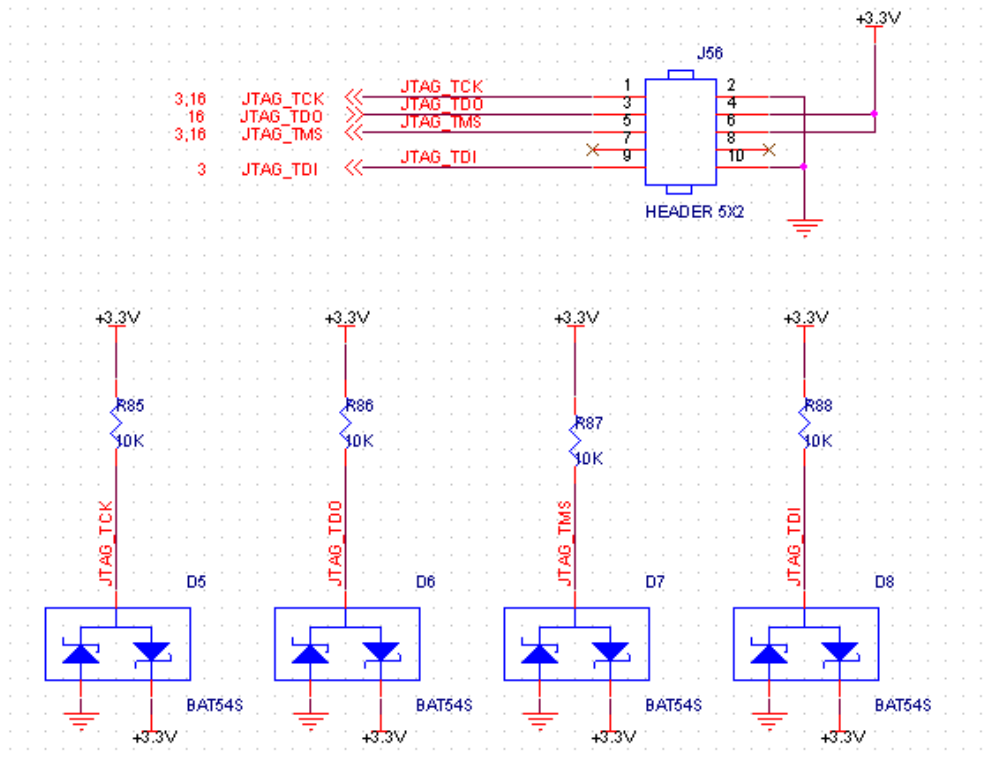
Figure 3-14-1: JTAG Interface Schematic
