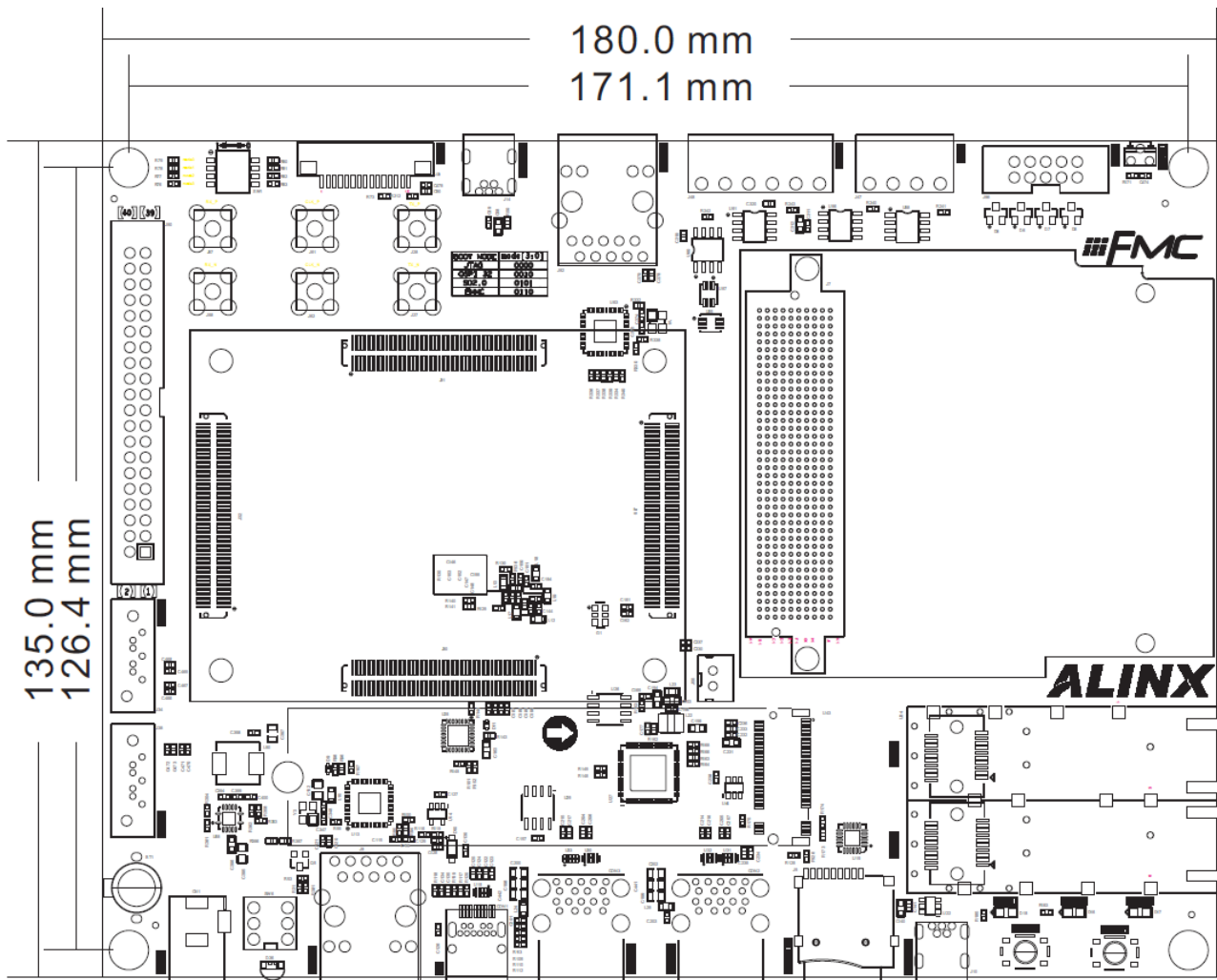
Figure 3-22-1: Carrier Board Form Factors
