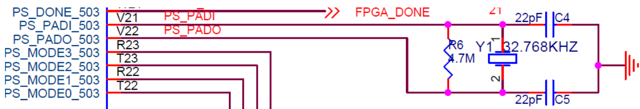
Figure 2-6-2: Passive Crystal Oscillator for RTC
