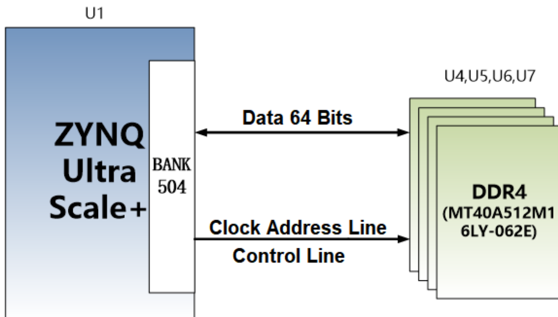
Figure 2-3-1: PS DDR4 DRAM schematic diagram
