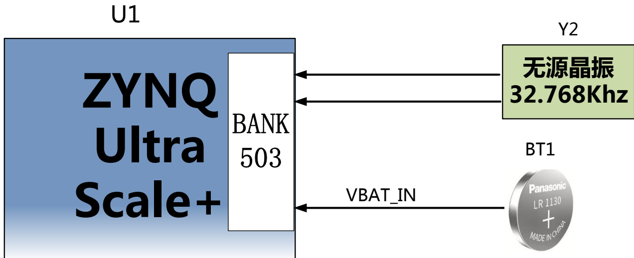
Figure 3-15-1: RTC Schematic
