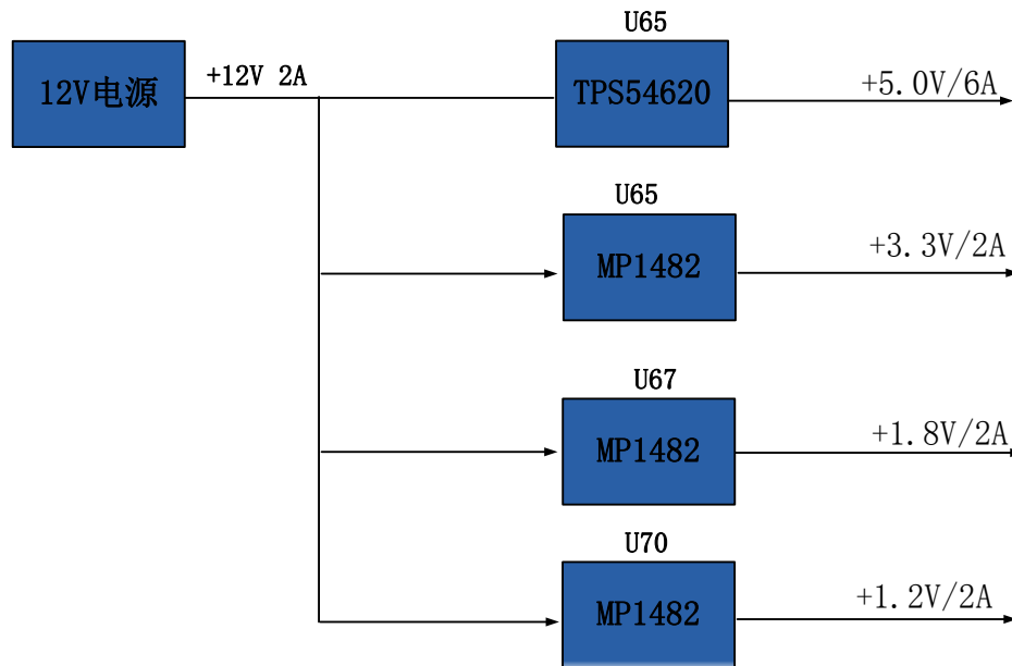
Figure 3-20-1: Carrier Board Power Schematic
