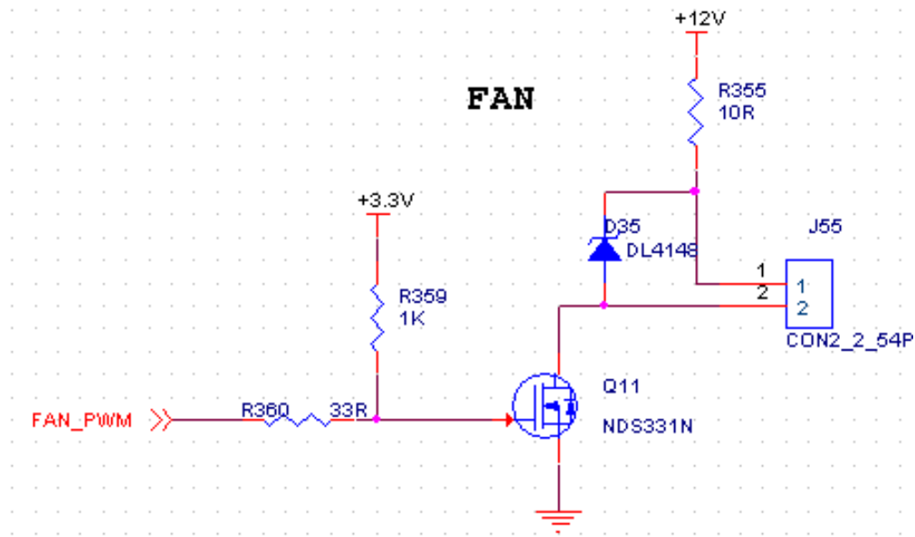
Figure 3-21-1: Fan Design Schematic
