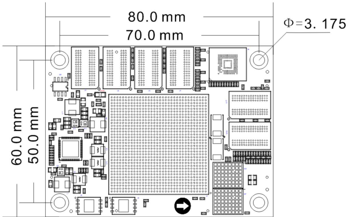
Figure 2-8-1: ACU15EG Core Board Form Factors
